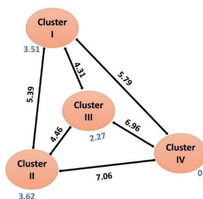
Fig. 3. Average intra and inter-cluster distances ( D^2 ) among nineteen mungbean mutants/varieties in four clusters. Here, intra-cluster distance values are present in blue and inter-cluster distances in black.
