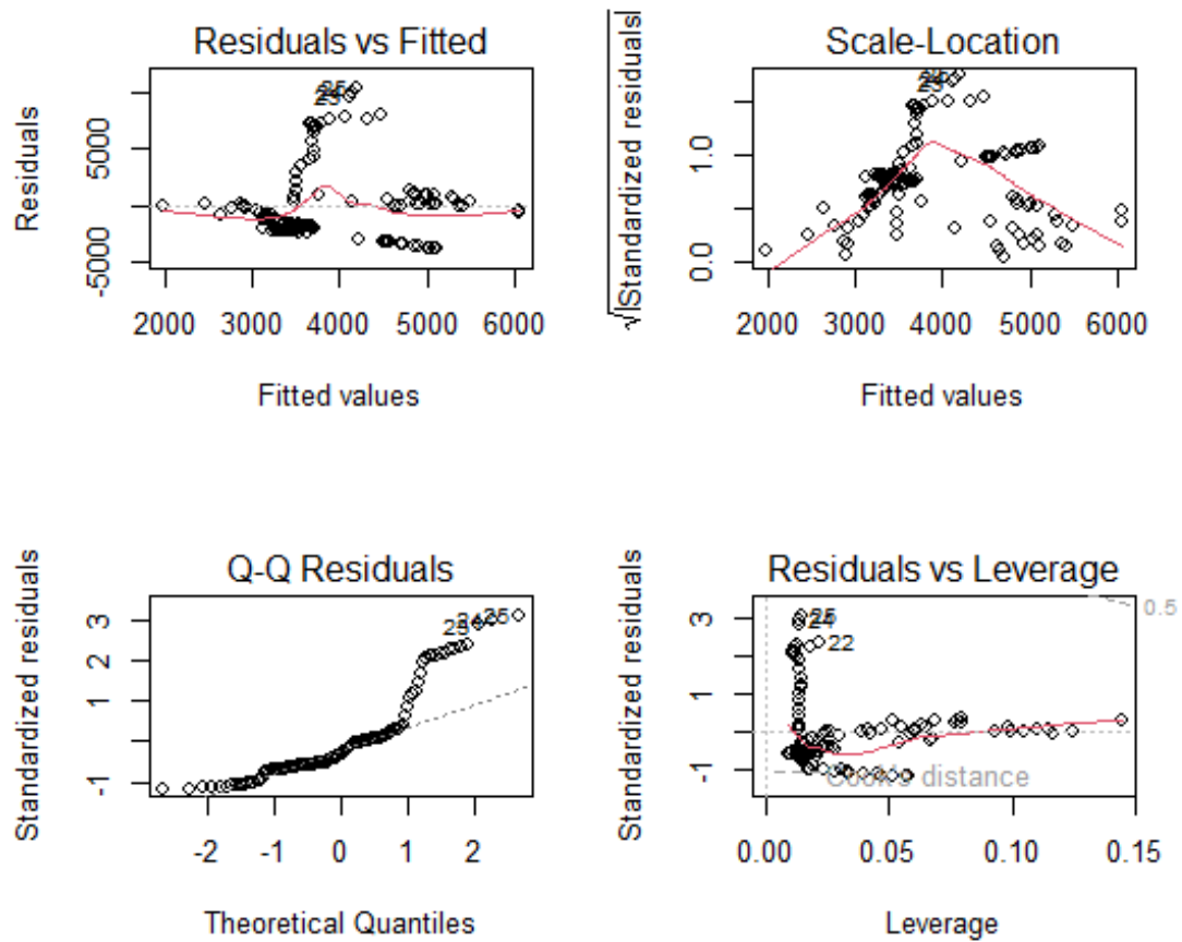
Figure 7. Residual analysis of the energy management systems dataset.
