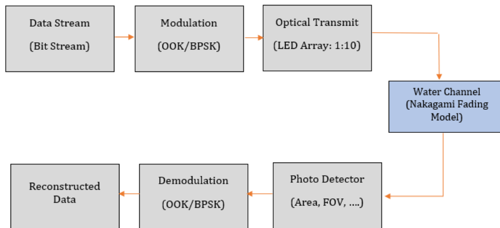
Fig. 1: UVLC system block diagram.
