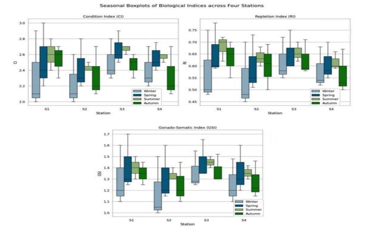
Fig. 2. Boxplots showing the seasonal variation of physiological indices (CI, RI, GSI) of Mytilus galloprovincialis during 2017
