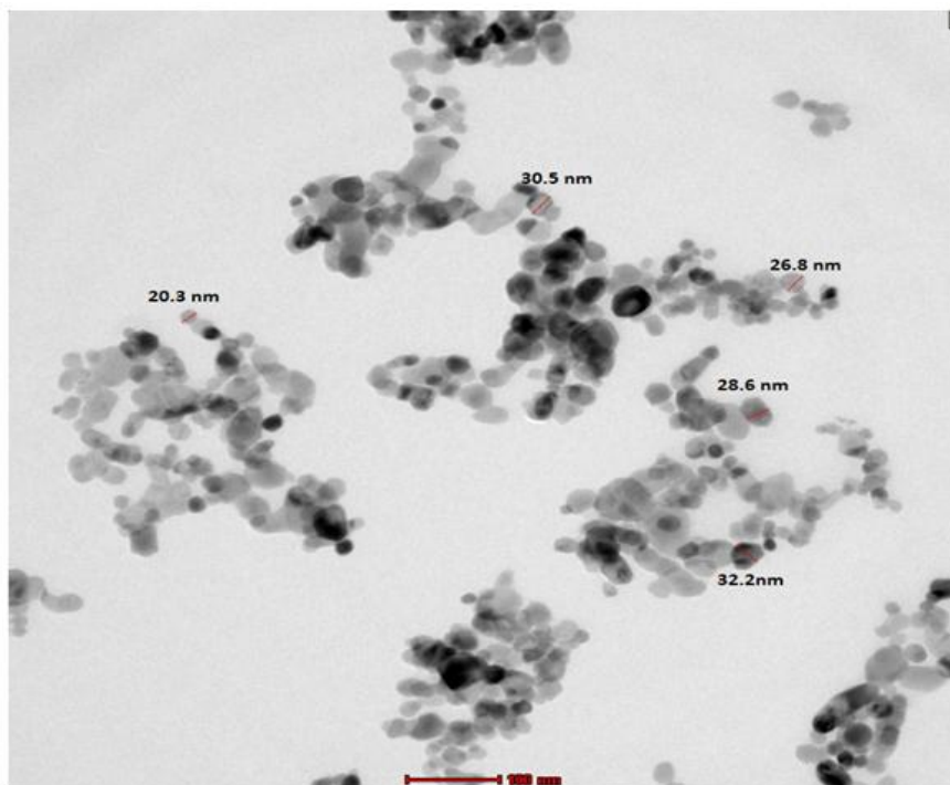
Figure 4. TEM image of the synthesized ZnO-NPs.
