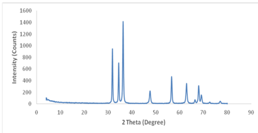
Figure3. The XRD pattern of the synthesized ZnO-NPs.
