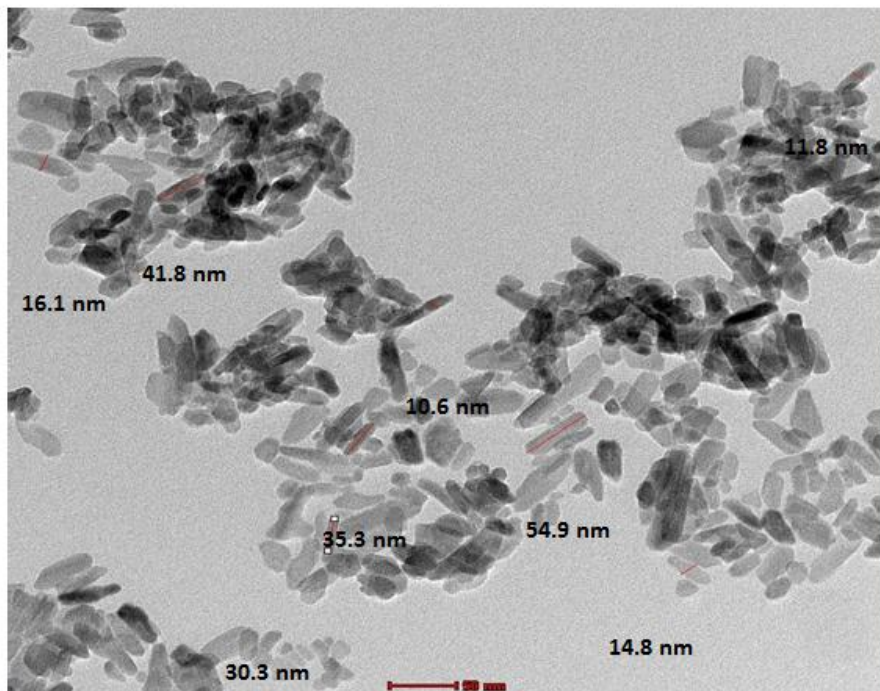
Fig.2. TEM image of HA-NPS powders synthesized.
