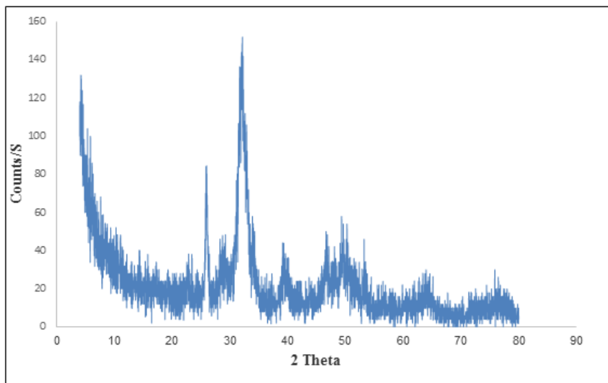
Fig. 1. XRD patterns of hydroxyapatite (HA) powders synthesized.
