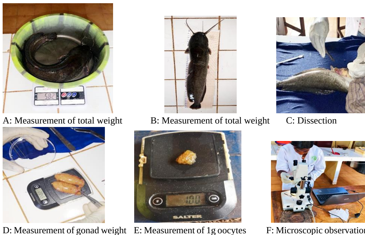
Fig. 3. Procedure for measurement, dissection, and microscopic observation
