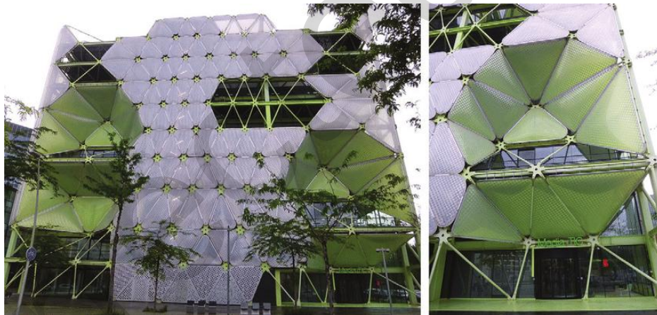
Fig. 2: Elevation: Shows the modular, inflatable ETFE cushions in detail, illustrating how they act as an adaptive outer layer.
