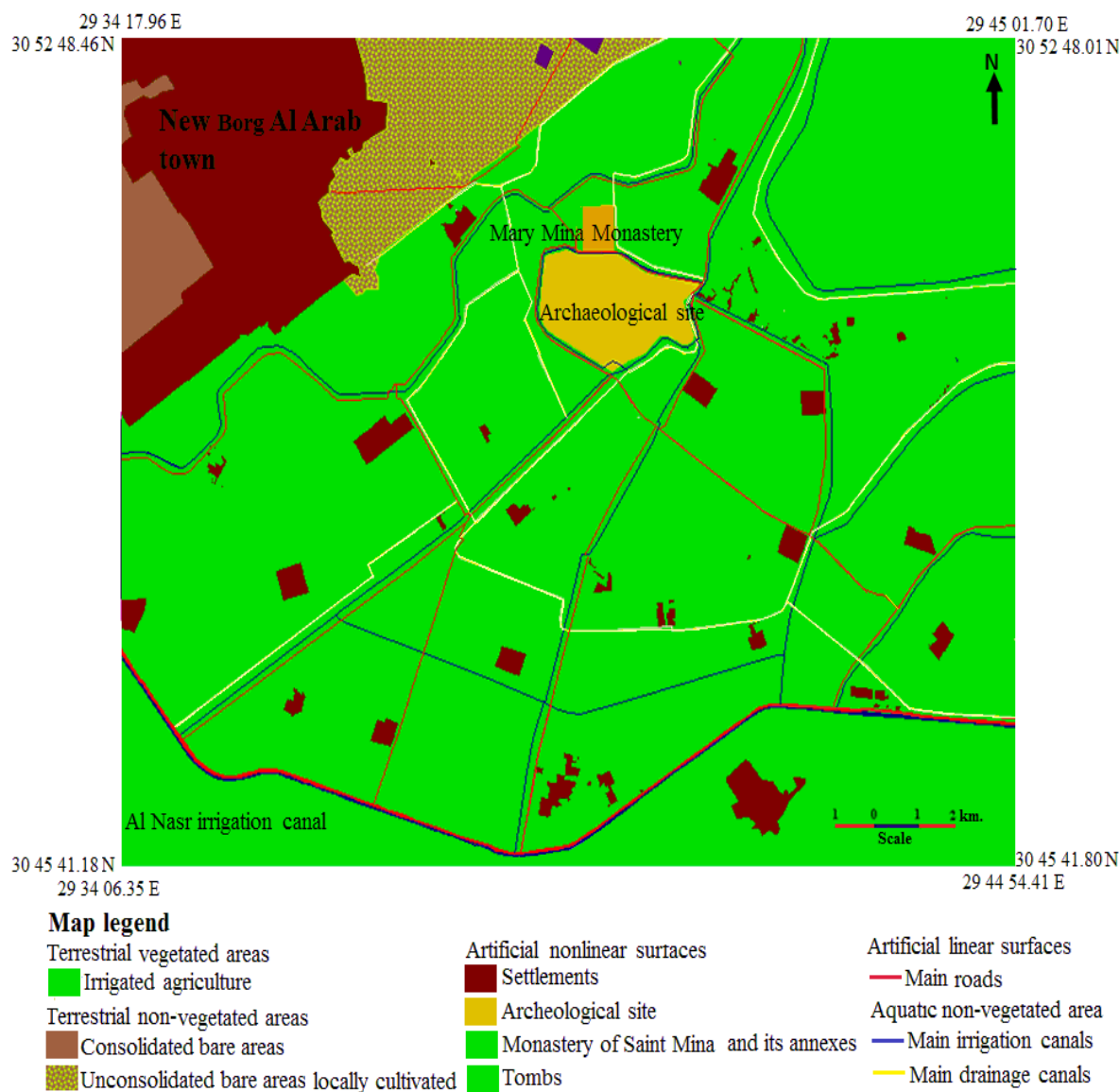
Figure 2. The geographic distribution of land cover classes in the study area
