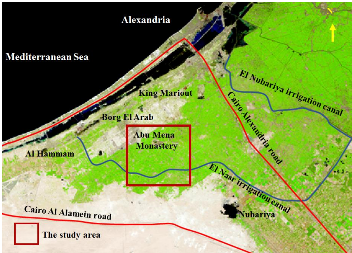
Figure 1 Location map of the study area allocated on sub seen of Sentinel 2 2025
