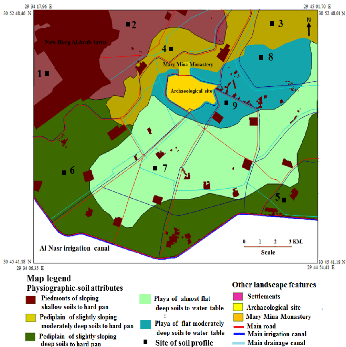
Figure 5 Physiographic features in the study area
