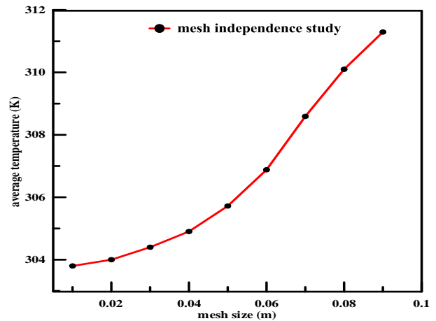
Fig (4) Parametric study on the mesh size
