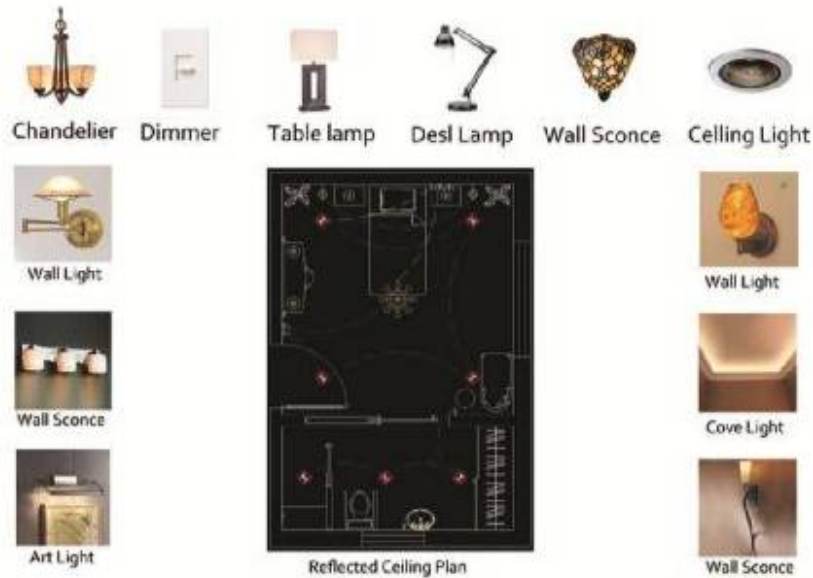
Figure 15: Men's Unit lighting plan & lighting fixtures.
