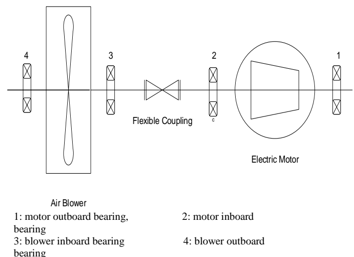
Fig. 1 Schematic diagram of atomization air blower
