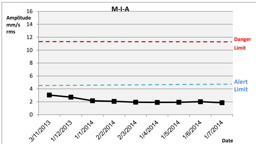
Fig. 14 Motor inboard bearing overall values in axial direction after machine rectification
