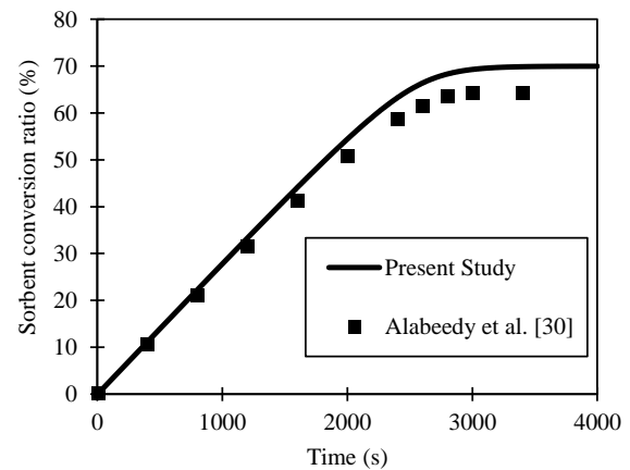
Fig. 10 Sorbent conversion ratio with time
