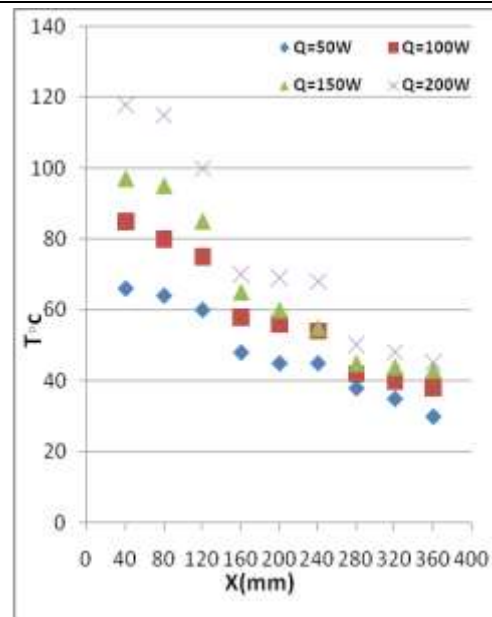
Fig(4) Effect of input heat on heat pipe wall temperature distribution for FR = 0.5 and uncoated wick.
