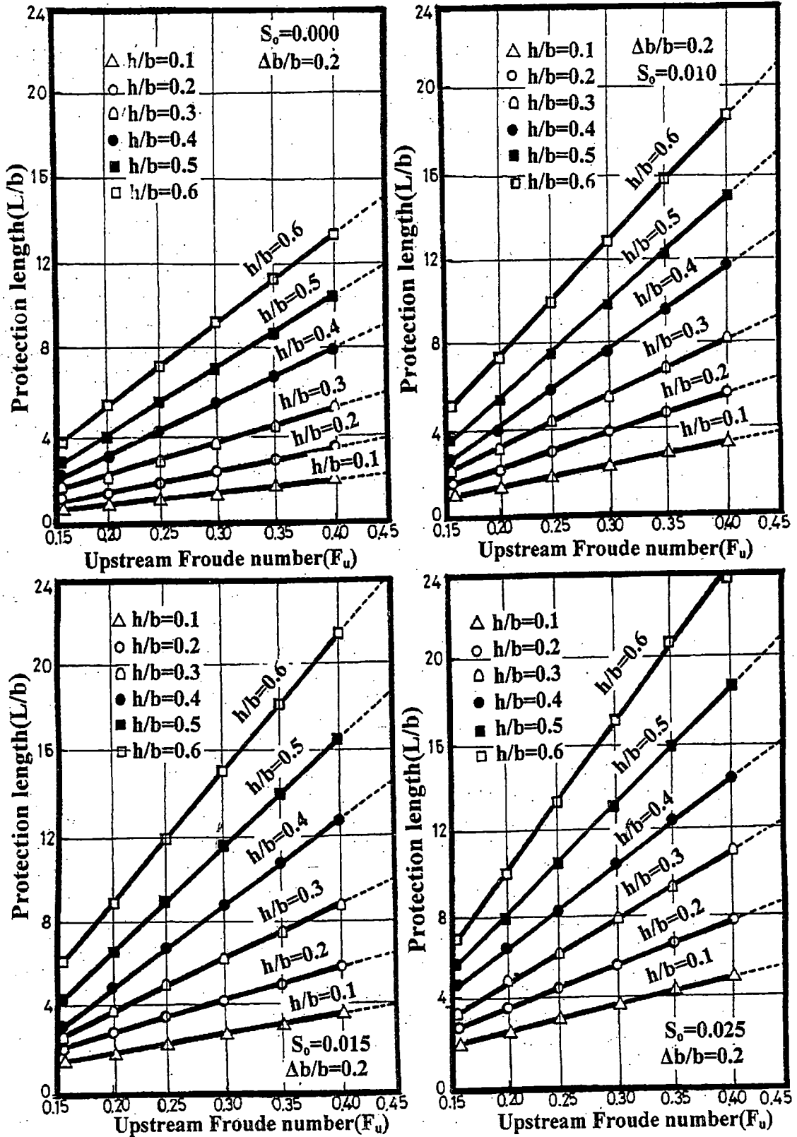
Fig.(6) Variation of upstream Froude number F_u with protection length L/b for different relative height h/b at different bed slope S_o at at fixed contraction ratio \Delta b/b = 0.2 .
