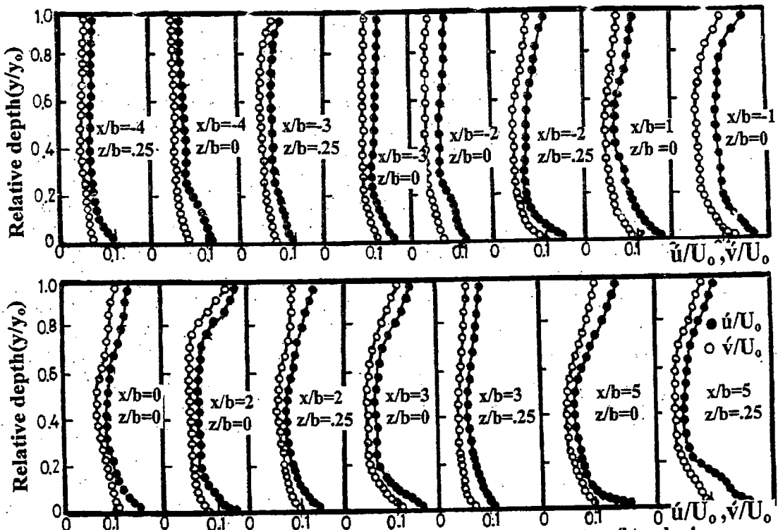
Fig.(8)Variation of streamwise and vertical components of turbulence intensities \dot{u}/U_0 and \dot{v}/U_0 with relative water depth y/y_0 at different locations at contraction ratio \Delta b/b=0.3 and h/b=0.3 for Q=40 lit./s.
