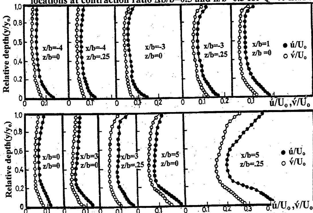
Fig.(9)Variation of streamwise and vertical components of turbulence intensities \dot{u}/U_0 and \dot{v}/U_0 with relative water depth y/y_0 at different locations at \Delta b/b=0.3 and relative height h/b=0.3 for Q=15 lit./s.
