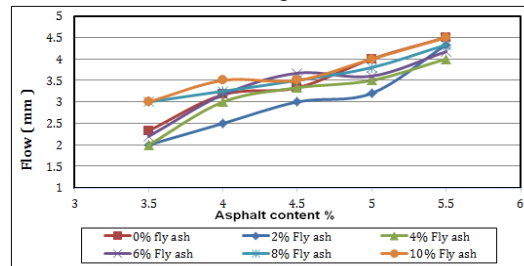
Fig. 11. Variation of Flow value with AC % modified by F.A
