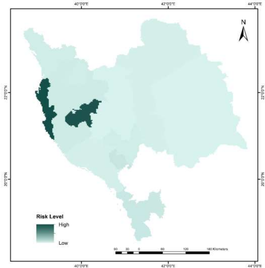
Fig. 3. GWR prediction model of COVID-19 risk, based on population and population density
