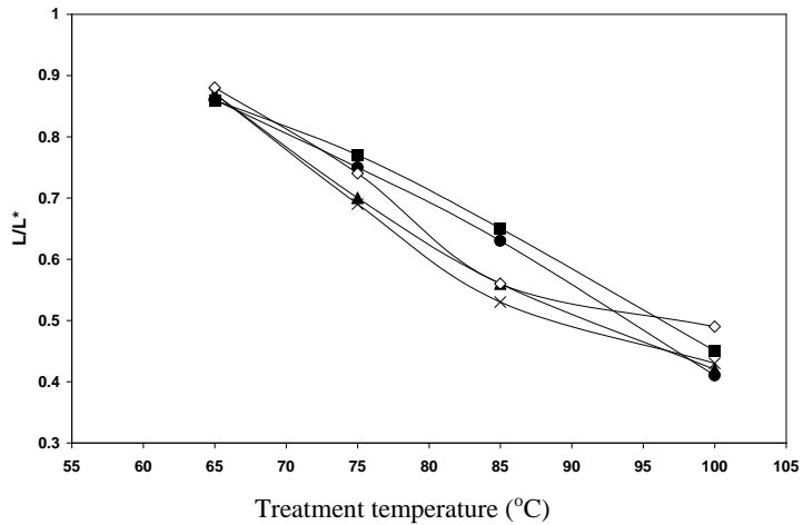
Figure 6: Effect of treatment temperature & type of substrates on the lightness of the fabric
