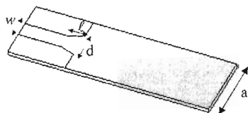
Fig. 2. Configuration of the transition of microstrip line to rectangular waveguide
