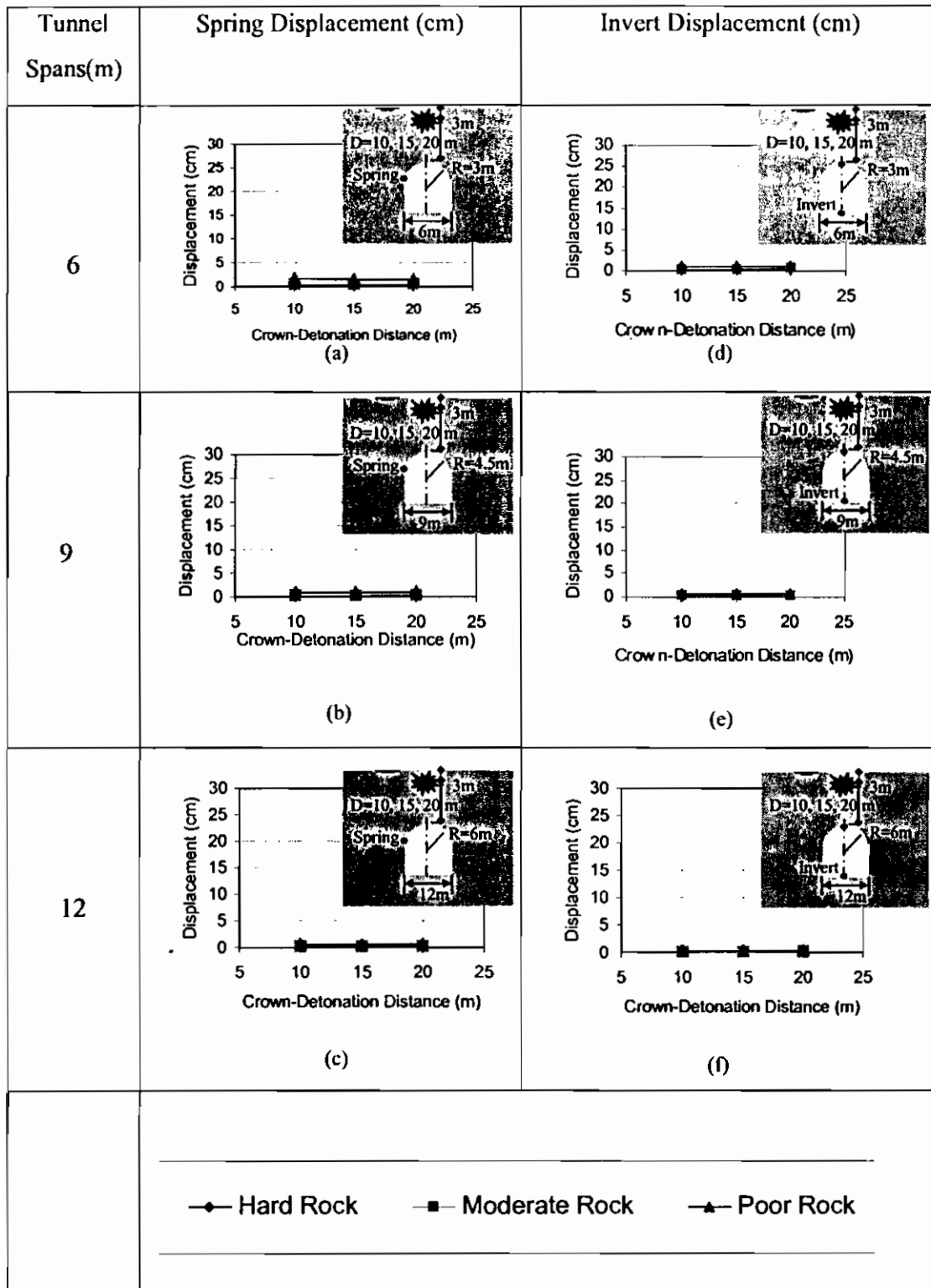
Fig. (7) Peak displacement of spring and invert point versus crown detonation distance for different tunnel spans and rock type
