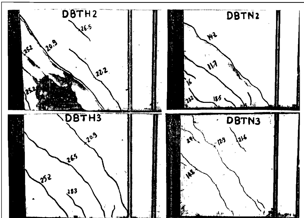
Fig. (6): Photographs of the crack patterns of some the tested NSC and HSC deep beams with L/h=1.0 .
