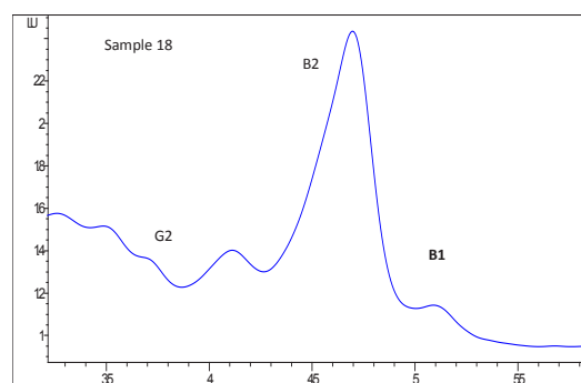
Fig. 4. HPLC analysis of aflatoxins in cultural extract of Aspergillus flavus isolated from wheat flour (strain 18) [Vertical axes represents wave length (w) and horizontal axes represents time in minutes (min)]
