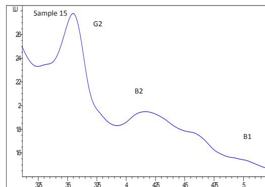
Fig. 3. HPLC analysis of aflatoxins in cultural extract of Aspergillus parasiticus isolated from wheat flour (strain 15) [Vertical axes represents wave length (w) and horizontal axes represents time in minutes (min)]
