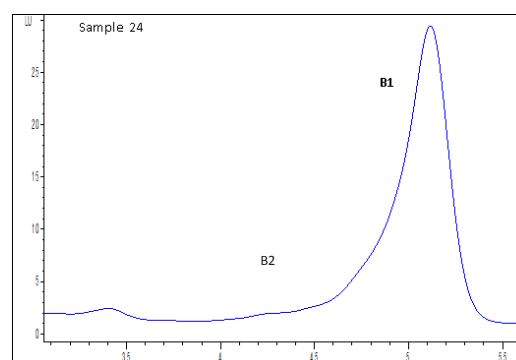
Fig. 5. HPLC analysis of aflatoxins in cultural extract of Aspergillus parasiticus isolated from wheat flour (strain 24) [Vertical axes represents wave length (w) and horizontal axes represents time in minutes (min)]
