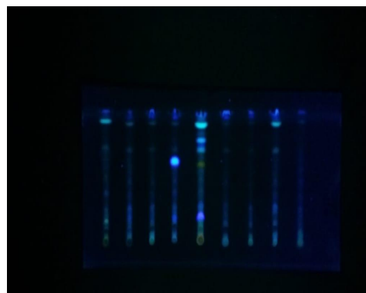
Fig. 1. Detection of aflatoxin production in Aspergilli isolates from wheat flour using thin-layer chromatography [Starting from left, isolate WH-AF21 to isolate WH-AF29 on the right]
