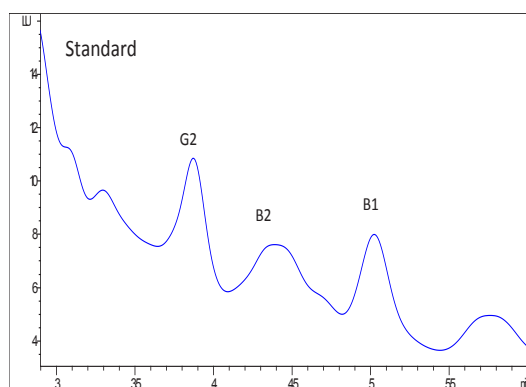
Fig. 2. Chromatograms obtained for a mixed aflatoxin standard (AFB1, AFB2 and AFG2) [Vertical axes represents wave length (w) and horizontal axes represents time in minutes (min)]
