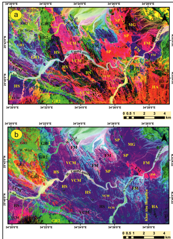
Fig. 6: PCA, a) 213, in RGB, b) 314, in RGB of landsat 8 (OLI), for abbreviations see (Fig. 4).
