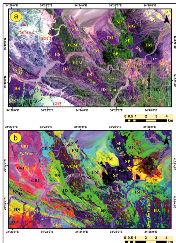
Fig. 5: Band ratios combinations: (a) 6/2, 4/3, 7/3 and (b) 7/6, 6/5, 4/2, in RGB of landsat 8 (OLI), for abbreviations see (Fig. 4).
