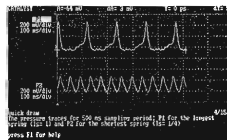
Fig.(3) Sample of Catalyst ® software for pressure wave form
