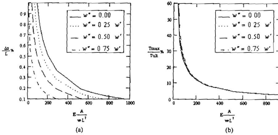
Fig. (4): The relation between the design parameters, in (10 \times 10) circular cable net with sag/span ratio of 3%: (a) the central deflections, (b) the maximum cable forces.
