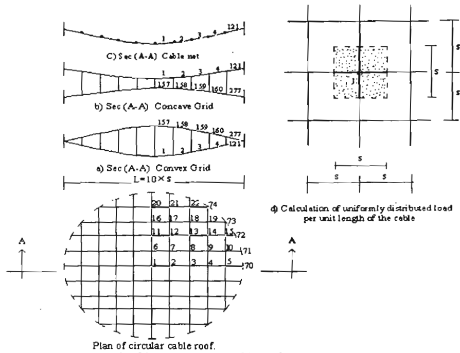
Fig. (2): Counter-stressed cable grid roofs.
