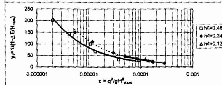
Figure (6) Relationship Between 1/(1-\Delta E/H_{dam}) and q^2/gH^3_{dam} for Different Step Configurations
