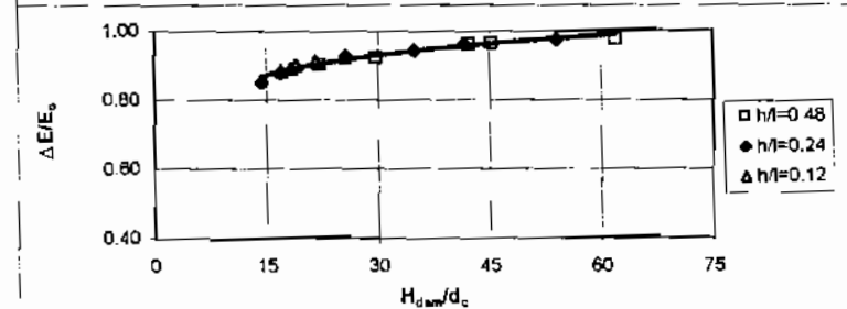
Figure (9) Nappe Flow Regime [\Delta E/E_0 - H_{dam}/d_c] Relationship, H_{dam}/d_c > 15
