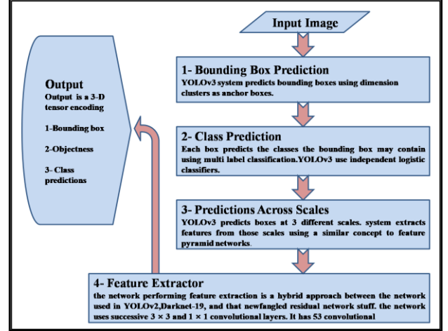
Figure 1: YOLOv3 layers specification and data flow
