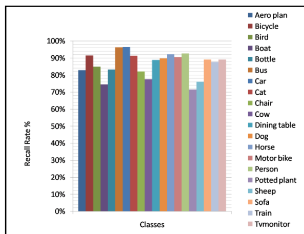
Figure 12: Recall Rate over Pascal 2007 classes
