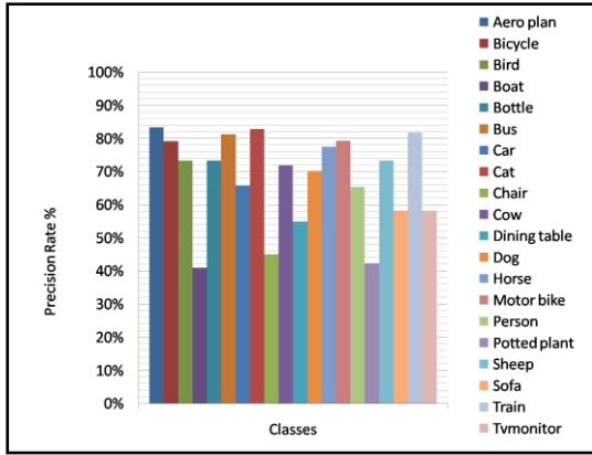
Figure 13: Precision Rate over Pascal 2007 classes
