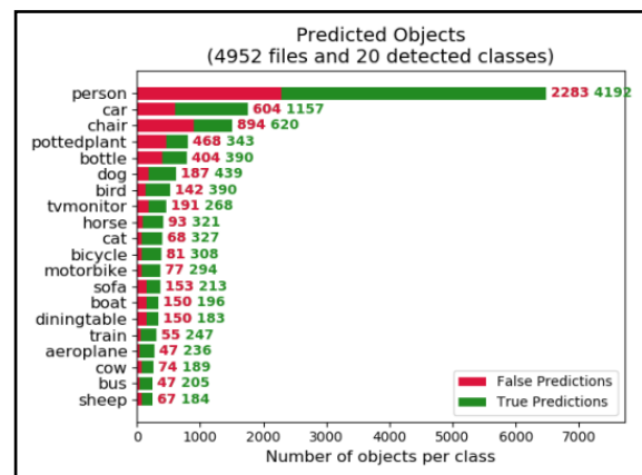
Figure 8: Test predictions rate over classes
