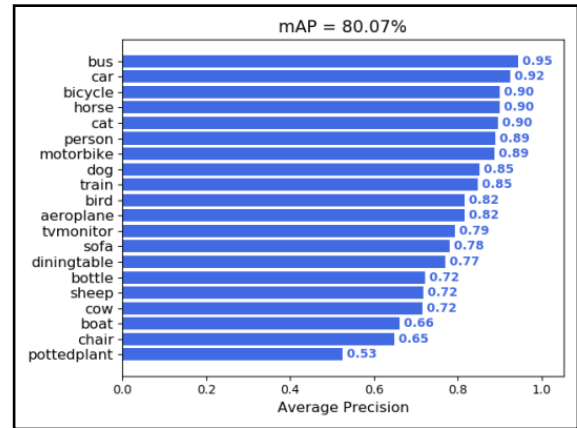
Figure 7: Average precision rate over classes
