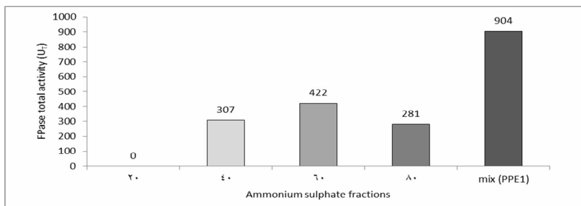
Fig. 5: LCEM partial purification by ammonium sulfate precipitation method
