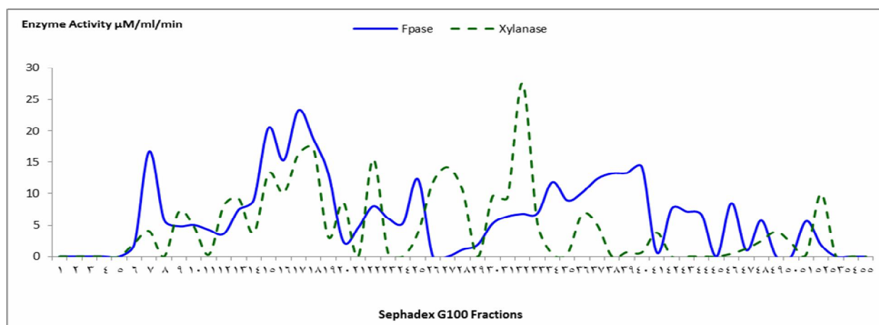
Fig. 6: Cellulolytic and xylanolytic activities of the separated fractions from partially purified enzyme mixture PPE1 on Sephadex G100 column (2.5 by 50 cm; Pharmacia Biotech Inc.) equilibrated with Tris-HCl buffer (50 mM, pH 7.5) buffer with flow rate of 10ml/15min.
