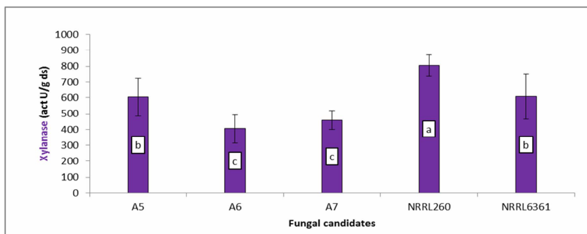
Fig. 4: Crude enzyme activities of the five xylanolytic fungi grown on SSF using pretreated RS as the sole carbon source. Highest results being designated as small letters (a, b, c) based on their specific LSD
