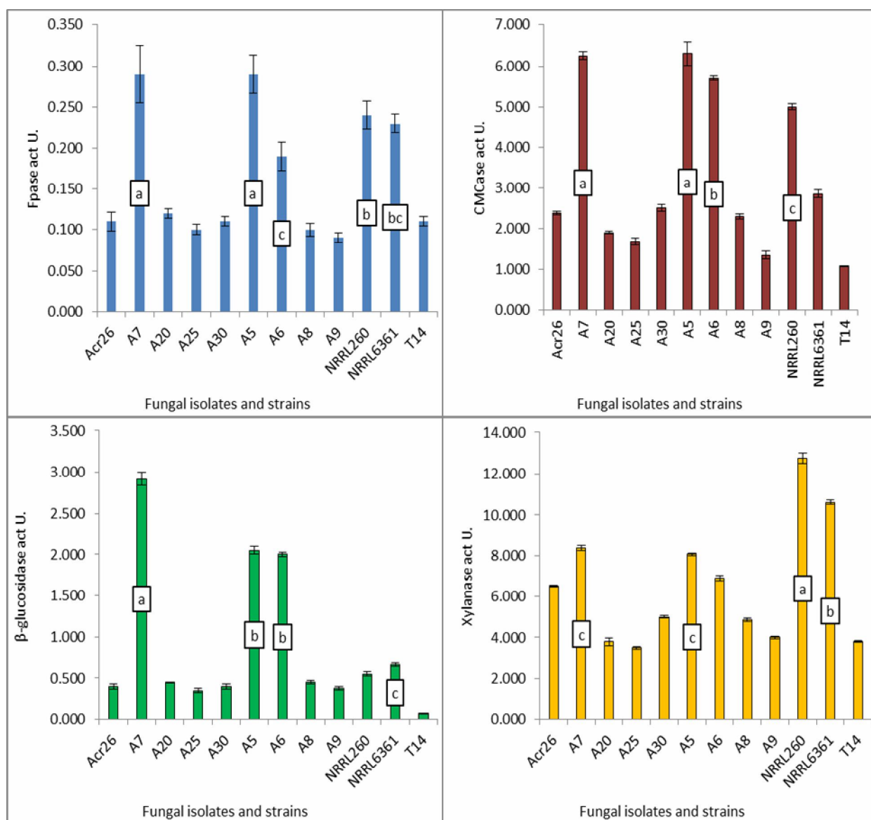
Fig. 2: Quantitative screening for cellulolytic and xylanolytic activities of the selected 12 cellulolytic fungi grown in SmF process on sugar cane bagasse (SCB). Best results being designated as small letters (a, b, c) based on their specific LSD.
