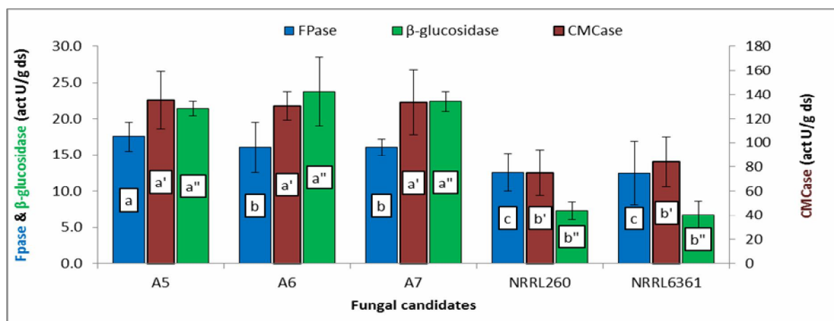
Fig. 3: Crude enzyme activities of the five cellulolytic fungi grown on SSF using pretreated RS as the sole carbon source. Highest results being designated as small letters (a, b, c) based on their specific LSD.
