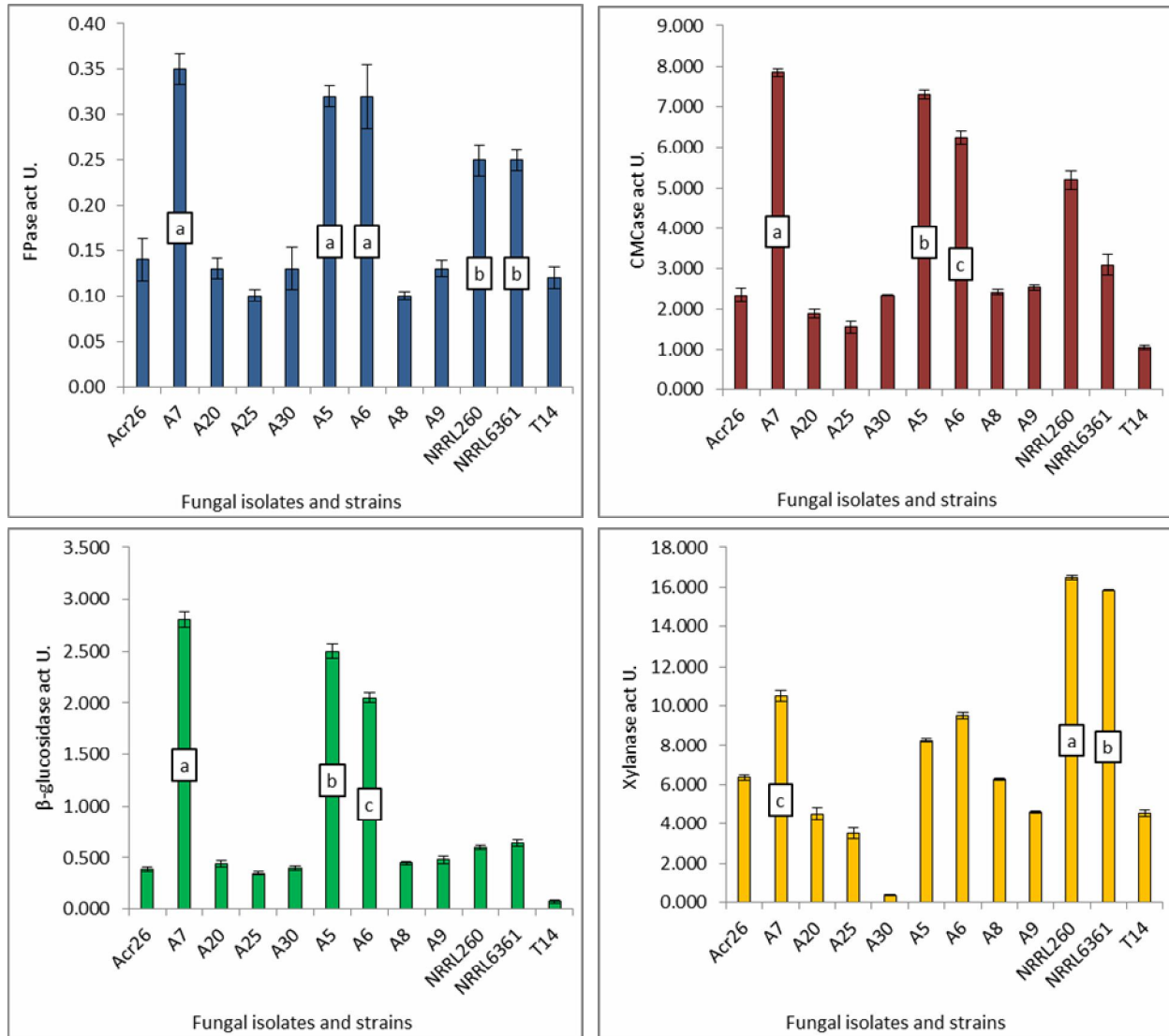
Fig. 1: Quantitative screening for cellulolytic and xylanolytic activities of the selected 12 cellulolytic fungi grown in SmF process on pretreated rice straw (RS). Best results being designated as small letters (a, b, c) based on their specific LSD.
