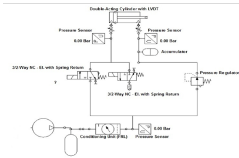
Fig. 2: Pneumatic circuit diagram
