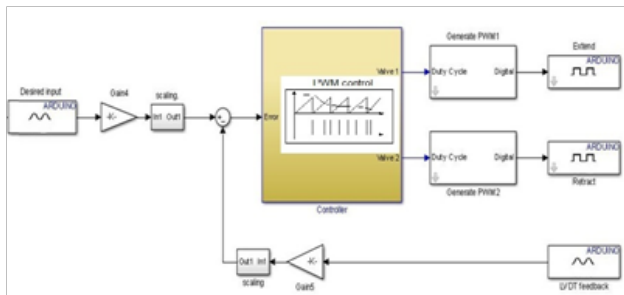
Fig. 4: Matlab ® Simulink scheme for modified PWM controller
