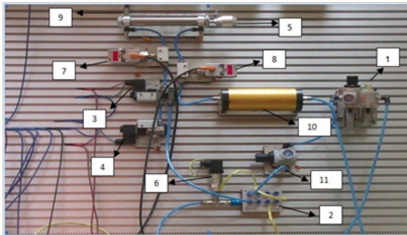
Fig. 1: Experimental pneumatic circuit used to test the modified PWM controller 1-Air preparation unit, 2-Air distributing unit, 3, 4- 3/2 Solenoid DCV, 5-Double acting pneumatic cylinder, 6-Pressure transducer no.1, 7-Pressure transducer no.2, 8- Pressure transducer no.3, 9-LVDT, 10-Accumulator, 11-Pressure regulator.
