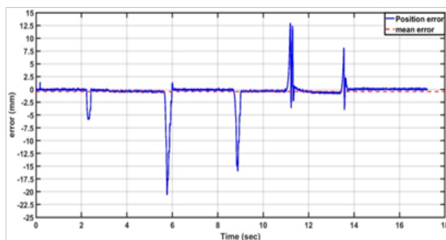
Fig. 9: Position error using modified PWM algorithm at P_{ac}= 4 bar.
