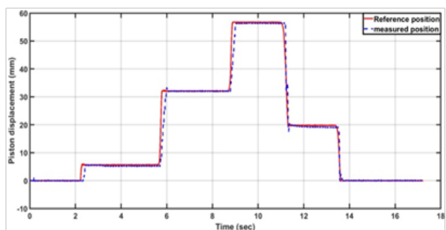
Fig. 8: Actuator response at P_s=4 bar and P_{ac}=4 bar.
