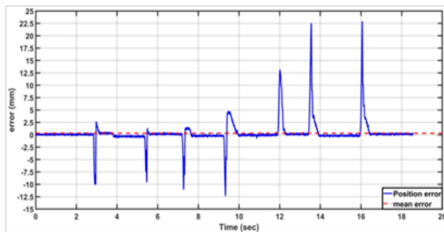
Fig. 7: Position error using modified PWM algorithm at P_{ac}=2.5 bar.
