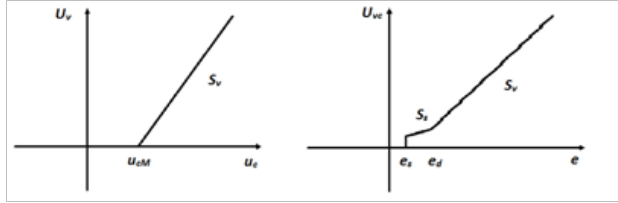
Fig. 3: Dead-zone characteristic (left), Graphical representation of DZC (right).
