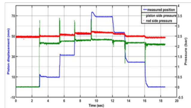
Fig. 6: Actuator response vs. pressure response with modified PWM control algorithm
