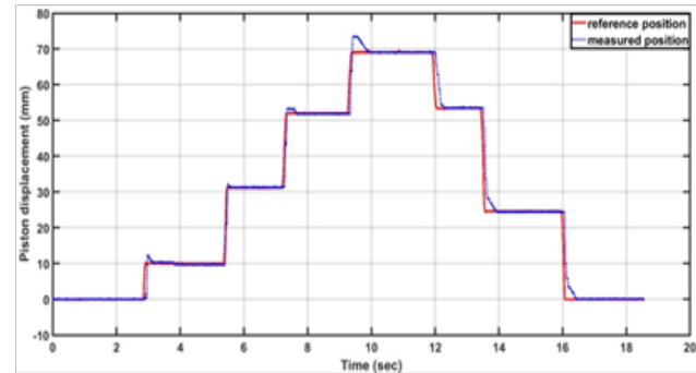
Fig. 5: Actuator response using modified PWM algorithm at P_{ac} = 2.5 bar
