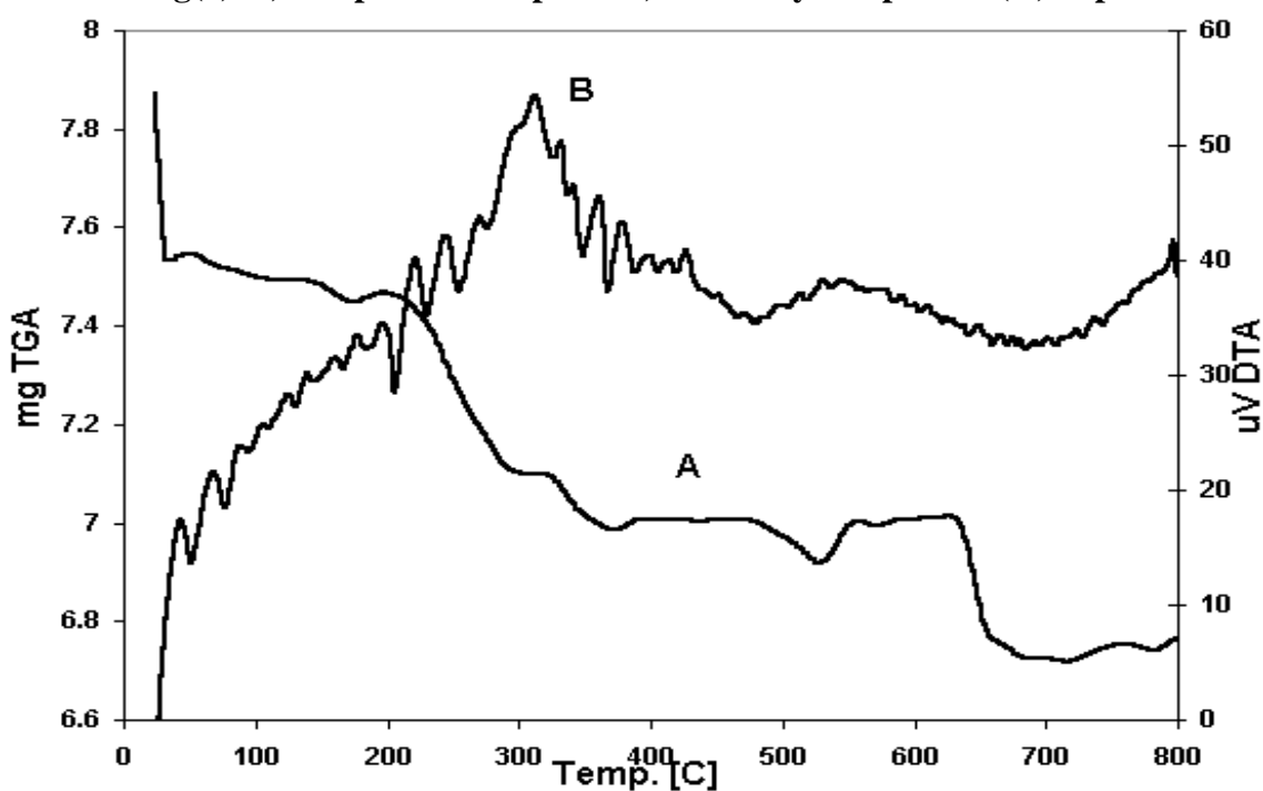
Fig.(6): A) Thermogravimetric analysis of Fe(II)-cap binary complex and B) its differential thermal analysis.
