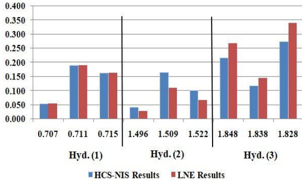
Figure 4: En-Values between HCS-NIS Results and LNE Results
