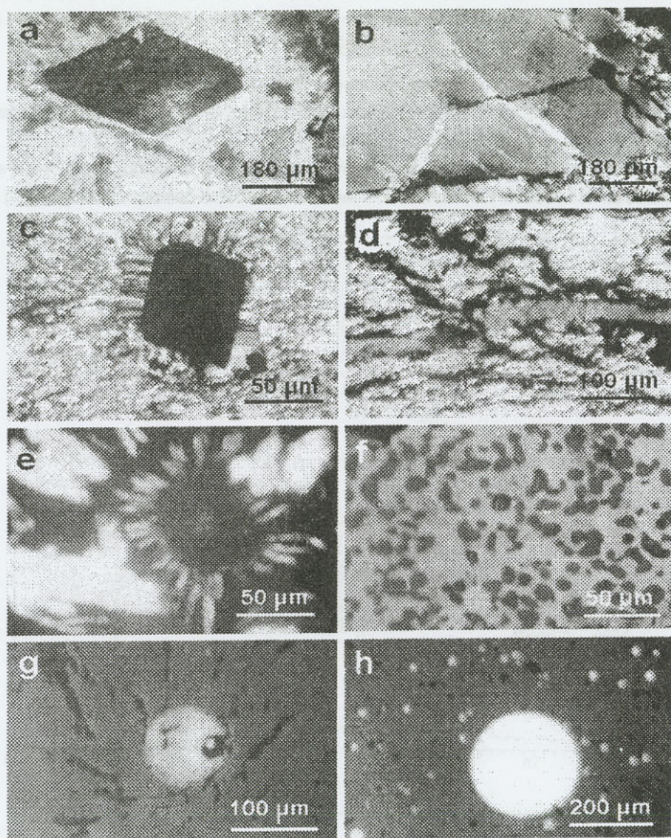
Fig. 4: a) Perfect actinolite rhomb in altered metadacite, P.P.L. b) Micro-conjugate fracturing of coarse quartz clast due to shearing, C.N. c) Resistant pyrite cube (black) showing strain shadow around as an indication of shearing, C.N. d) Paratacamite veinlet in highly hematitized metadacite, P.P.L. e) Radiating Fe-Mn silicate rods growing on a glass base in copper slag, P.P.L. f) Impure native copper showing numerous droplets of silicate and relict chalcocite, copper slag, reflected-light, P.P.L. g) Rusty copper prill showing fresh excentric native copper core, copper slag, reflected-light, P.P.L. h) Two different sizes of completely fresh copper prills in the copper slag, reflected-light, P.P.L.
