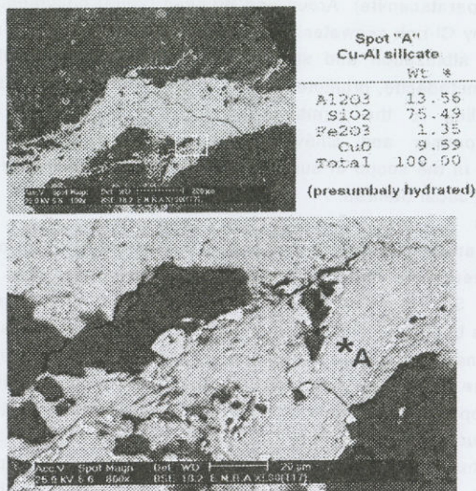
Fig. 10: SEM image showing dense secondary copper veinlet in altered metadacite. The EDX microanalysis of this hydrated Cu-Al phase is also given
