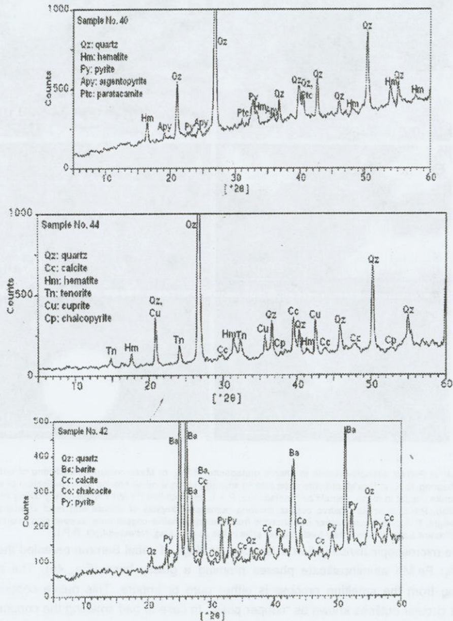
Fig. 3: XRD charts of some analyzed samples from the mineralized shear zone at Jabal Samran
