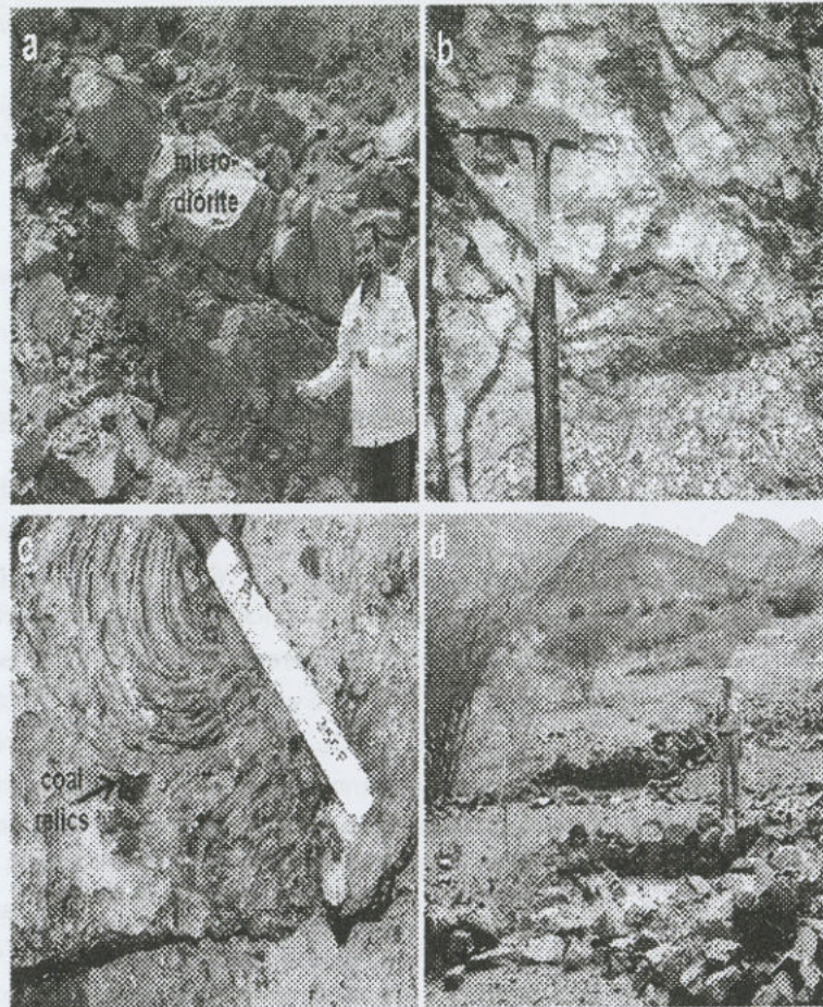
Fig. 2: a) Microdiorite intruding hydrothermally altered metavolcanics. b) Hydrothermal alteration of metadacite viz. hematitization. c) Rope-like surface of ancient copper slag. Notice the presence of relict charcoal. d) Ruins of ancient labour houses probably dated back to the time of Abbasiyeen.
