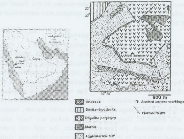
Fig. 1: Location map and geology of Jabal Samran area (modified after Ba-Battat, 1982)
