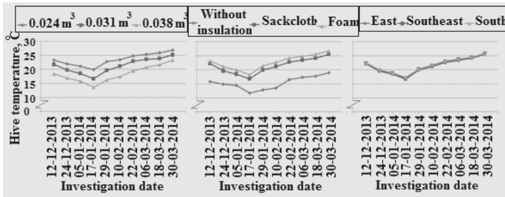
Fig. 5. Effect of the internal hive size, insulator type and hive entrance direction on hive temperature, °C
