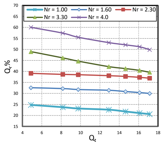
Fig. (3): Relationship between the Discharge Ratio ( Q_r ) and the total discharge ( Q_t ) for different bed roughness ratios ( n_r )
