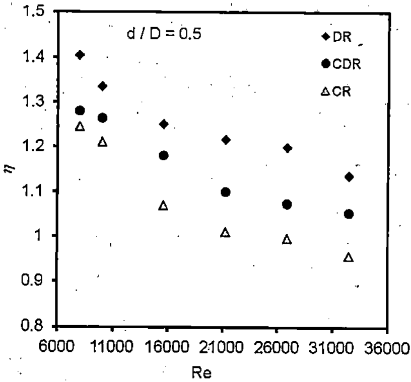
Fig. 11. Variation of the overall enhancement efficiency with Reynolds number for various conical ring arrays (CR/DR/CDR) at the diameter ratio d/D = 0.5 .
