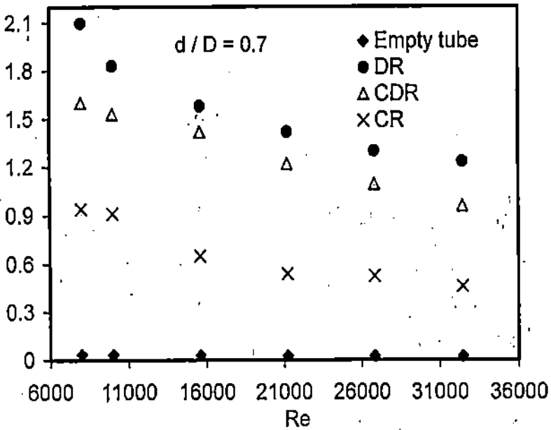
Fig. 10. Variation of friction factor with Reynolds number for various conical ring arrays (CR/DR/CDR) at the diameter ratio d/D = 0.7 .
