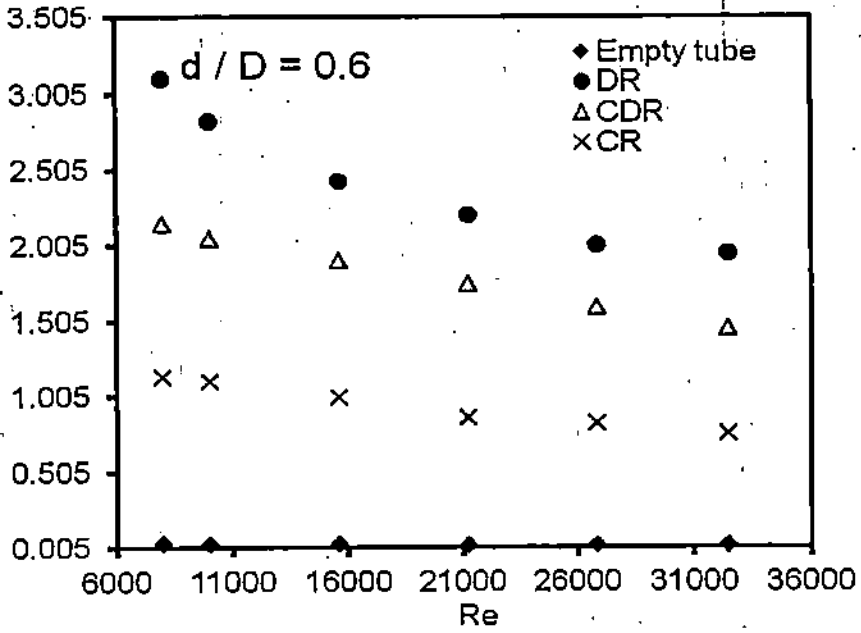
Fig. 9. Variation of friction factor with Reynolds number for various conical ring arrays (CR/DR/CDR) at the diameter ratio d/D = 0.6 .
