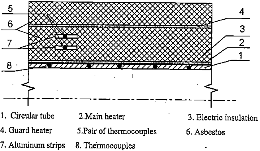
Fig.1b. Heaters arrangement
