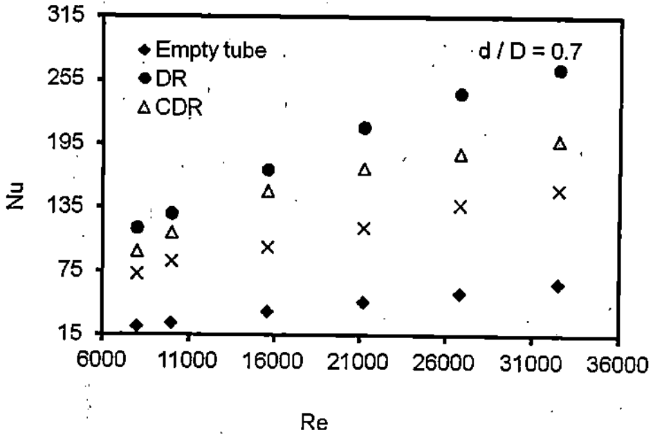
Fig. 7. Variation of Nusselt number with Reynolds number for various conical ring arrays (CR/DR/CDR) at the diameter ratio d/D = 0.7 .
