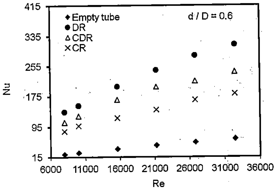
Fig. 6. Variation of Nusselt number with Reynolds number for various conical ring arrays (CR/DR/CDR) at the diameter ratio d/D = 0.6 .
