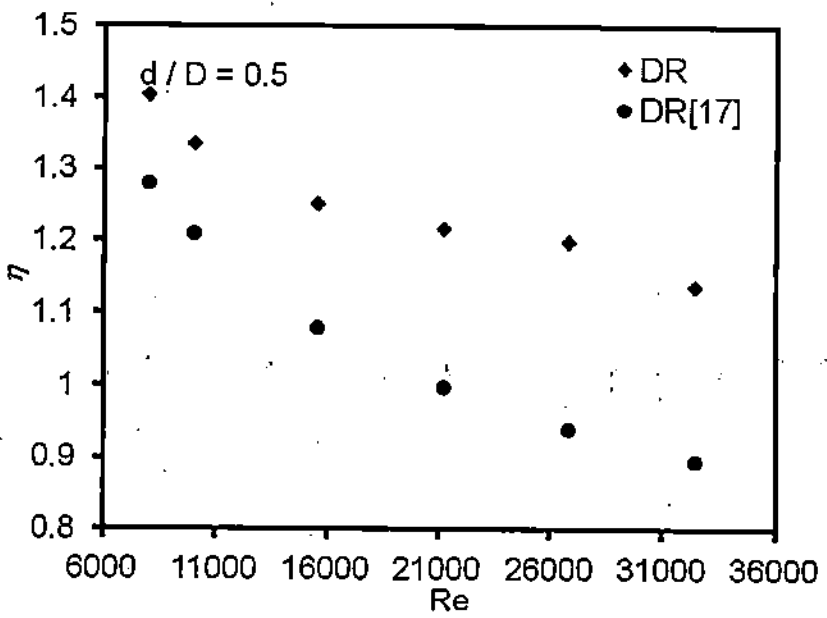
Fig. 20. Comparison of circular reference [17] and experimental value of the overall enhancement efficiency of conical rings with internal fins (DR) arrays at diameter ratio d/D=0.5 .
