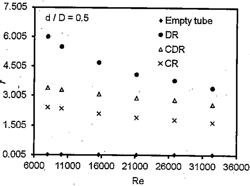
Fig. 8. Variation of friction factor with Reynolds number for various conical ring arrays (CR/DR/CDR) at the diameter ratio d/D = 0.5 .
