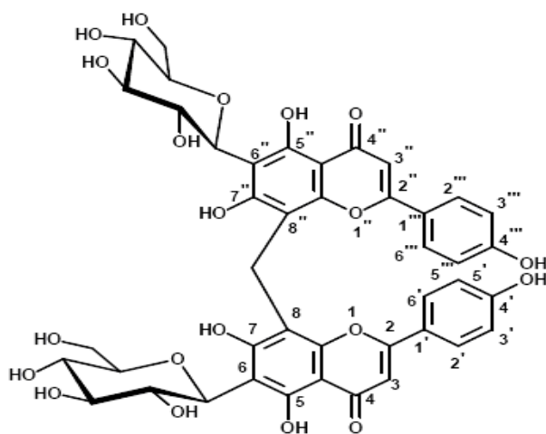
Biapigenin-(8,8'')-methylene-6,6''-di-C- \beta -D-glucopyranoside (1)
