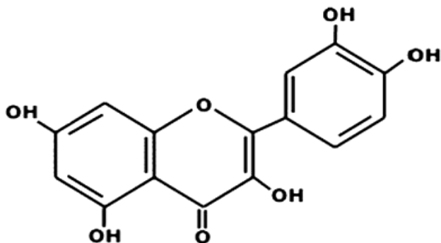
Apigenin (5)
