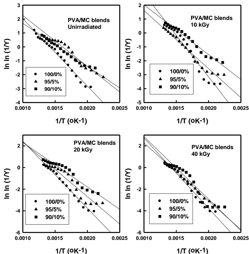
Fig .6. Plots of \ln \ln (1/Y) vs. 1/T where Y= (W_t-W_{\infty})/ (W_o-W_{\infty}) for gamma
