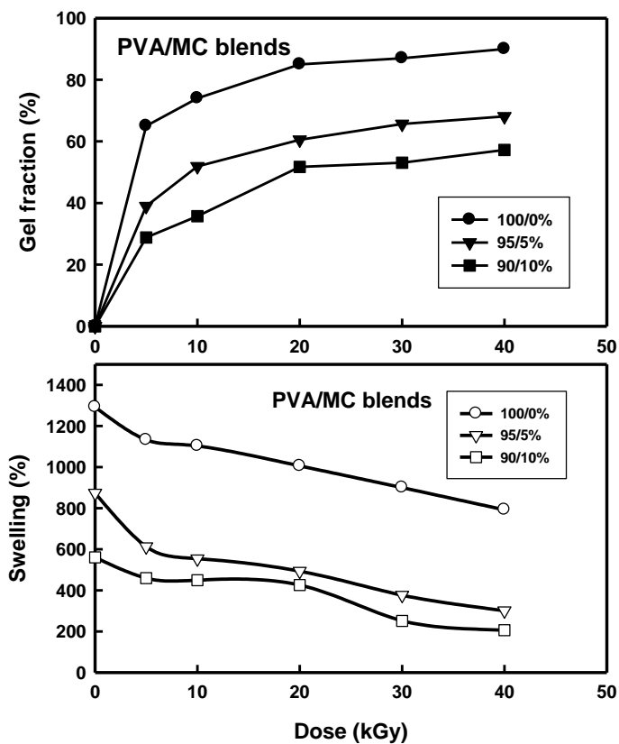
Fig.1. Effect of irradiation dose on the gel fraction (%) and swelling (%) in water at
