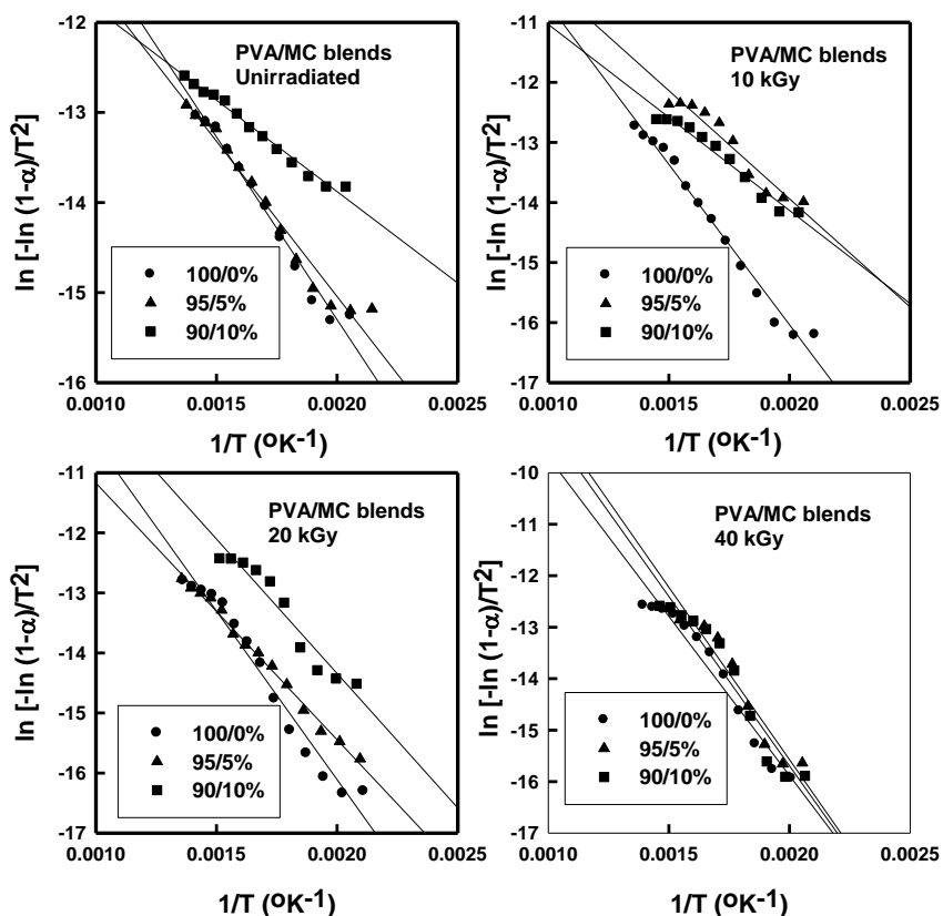
Fig.4. Plots of \log [g(\alpha)/T^2] vs. 1/T for gamma irradiated PVA/MC blends at different doses according to Coats–Redfern equation.
