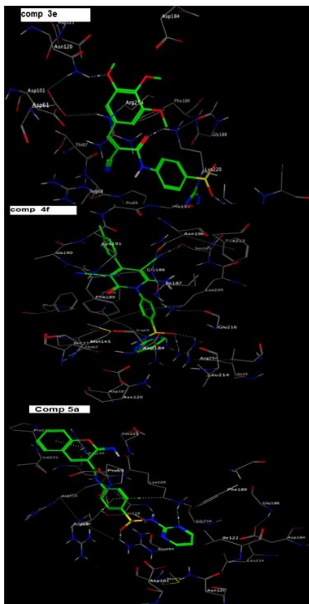
Figure (2): 3D representation of docking of compounds 3e , 4f and 5a in to the active site of 3TYE. Compound 3e shows three hydrogen bonds interaction with Ser221 , Lys220 and Asn120 . Compound 4f shows two hydrogen
