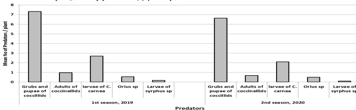
Fig. 5. Seasonal mean number of cotton aphid predators in eggplant field throughout two successive seasons 2019 and 2020
