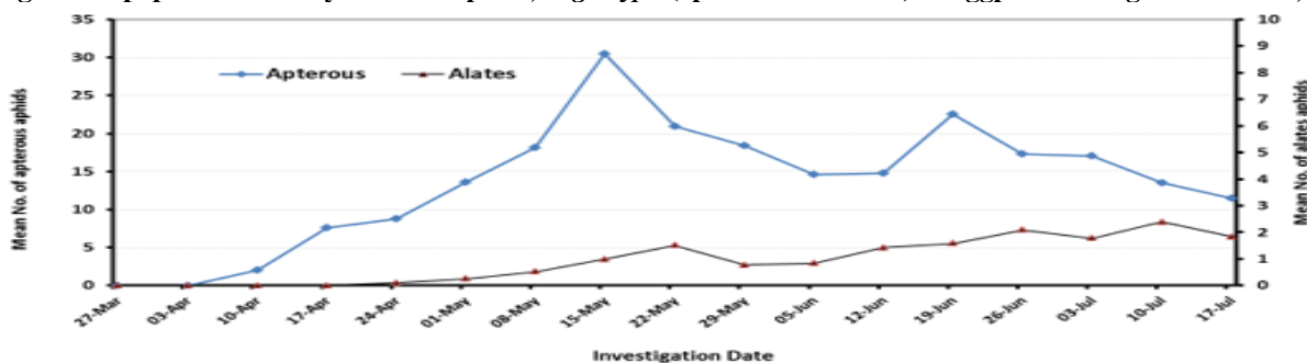
Fig. 2. The population density of cotton aphids, A. gossypii (apterous and alates) on eggplant during the second season, 2020
