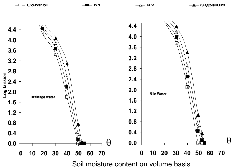
Fig 1-Effect of different fertilizer treatment and gypsum addition on soil moisture characteristic curves under different irrigation water types for studied soil samples
