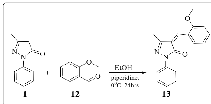
Scheme 9
