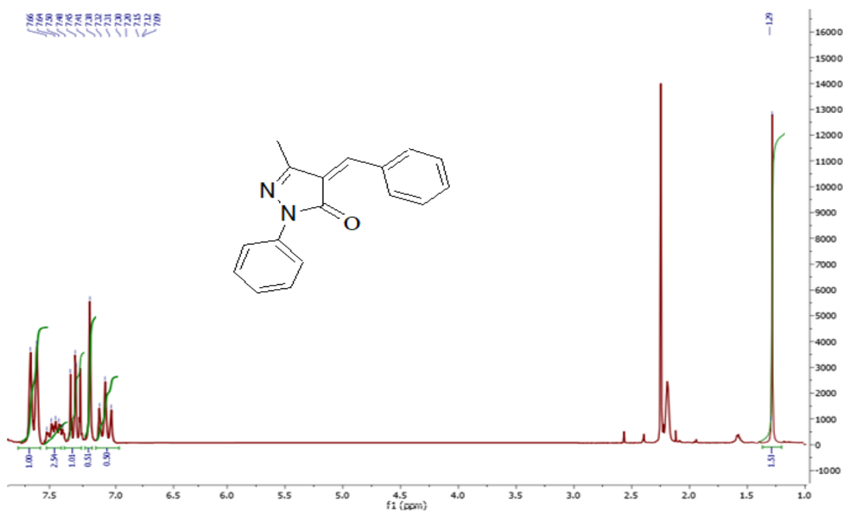
Fig. 2. 1 H-NMR(CDCl 3 , 400 MHz) for compound 3
