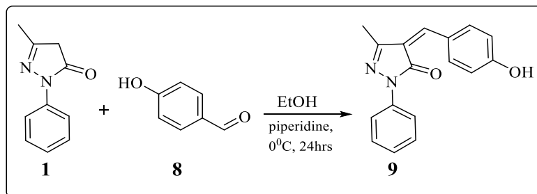
Scheme 7
