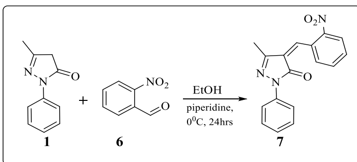
Scheme 6
