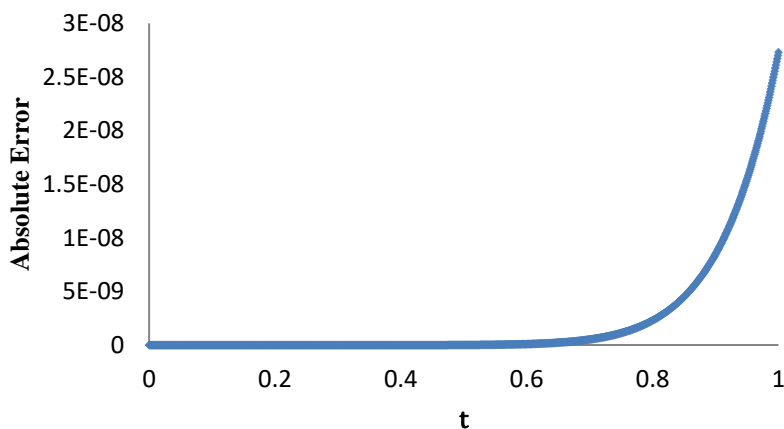
Fig.2. Absolute error graph for numerical and exact solutions versus t for \alpha = 1 and t = 0.5 .
