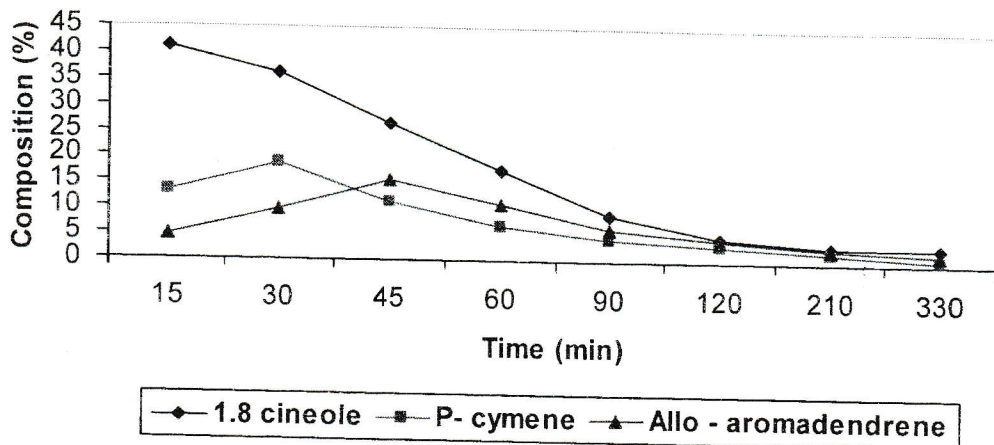
Fig.(3) : Main components % in oil fraction of E. gomphocephala obtained at time intervals during steam distillation (summer season2001).
