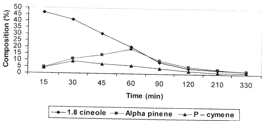
Fig.(3) : Main components % in oil fraction of E. gomphocephala obtained at time intervals during steam distillation (summer season2001).
