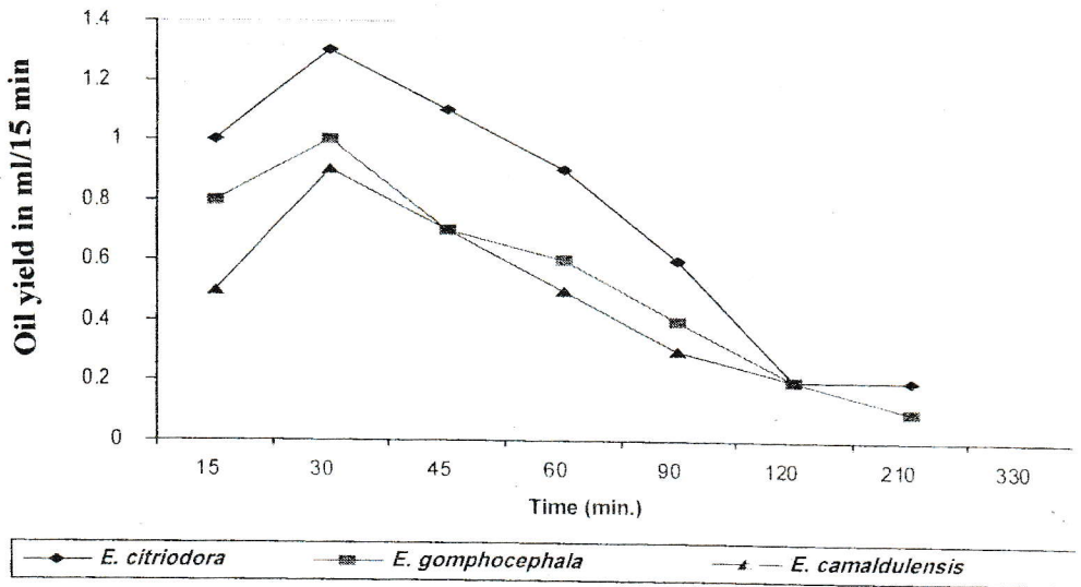
Fig. (1): Extracted oil in ml/ 15 min. during distillation .
