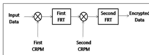
Fig. 1 Encryption process using FrFT_chaos function
