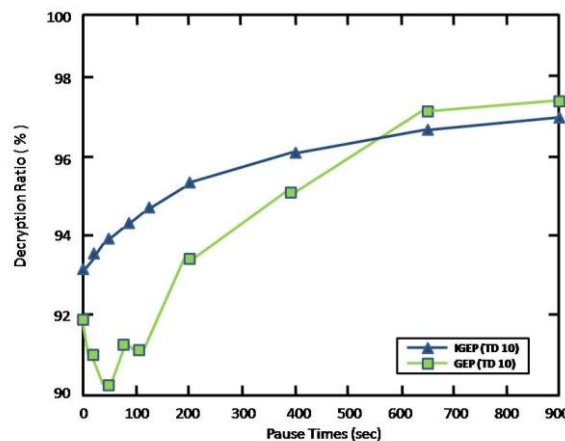
Fig. 7 Decryption ratio vs. mobility for 30 sources
