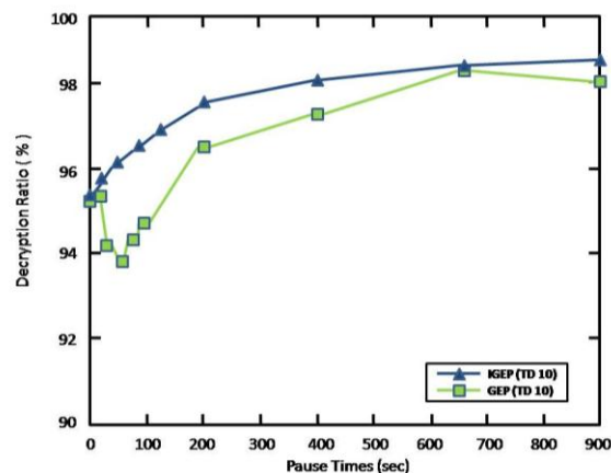
Fig. 5 Decryption ratio vs. mobility for 10 sources
