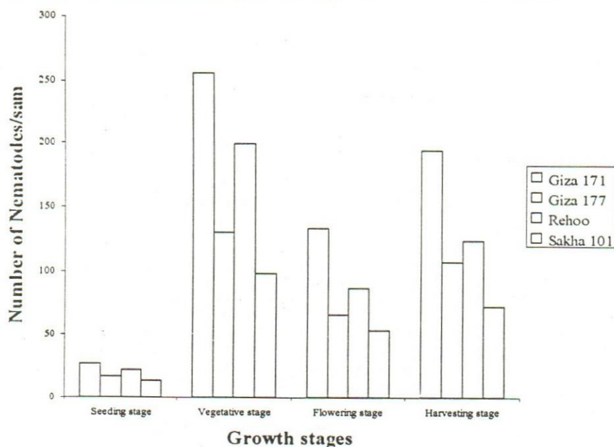
Fig. (1): Population changes of white-tip nematode Aphelenchoides besseyi on different stages of four rice cultivars grown in pots under outdoor conditions
