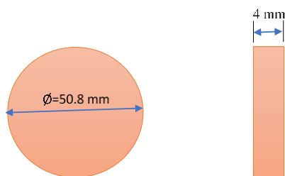
Fig 3. Diagram Sample for Standard Sample of Corrosion Testing.
