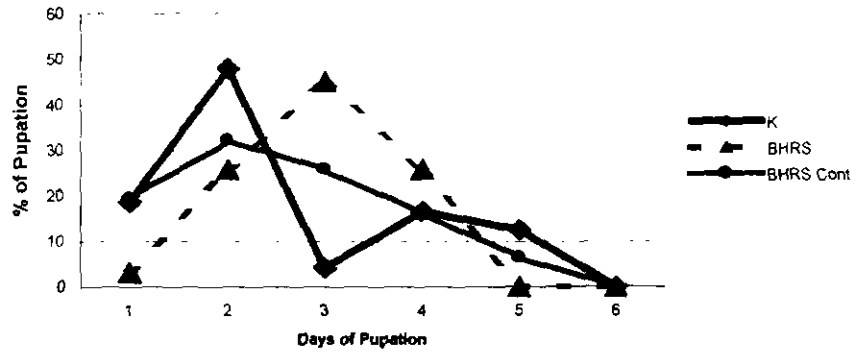
Fig 4 d BHRS
