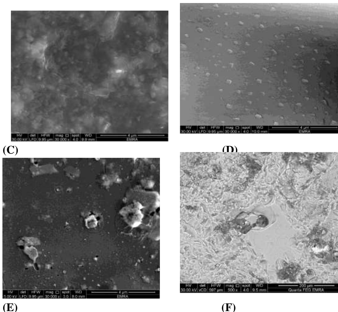
Fig 4 (A-F) SEM micrographs of the treated and untreated faience samples,(A) Wacker OH100, (B) TEOS, (C) Wacker OH100+Nanosilica, (D) TEOS+Nanosilica, (E) Nanolime and (F) untreatment sample standard .
