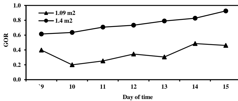
Fig. 6: Effect of contact surface area of packing on GOR.
