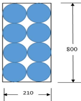
Fig. 3: Diagram for plastic fill packing spheres (dimensions in mm).
