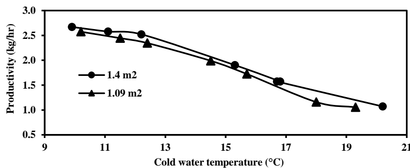
Fig. 7: Effect of cold-water temperature on productivity.
