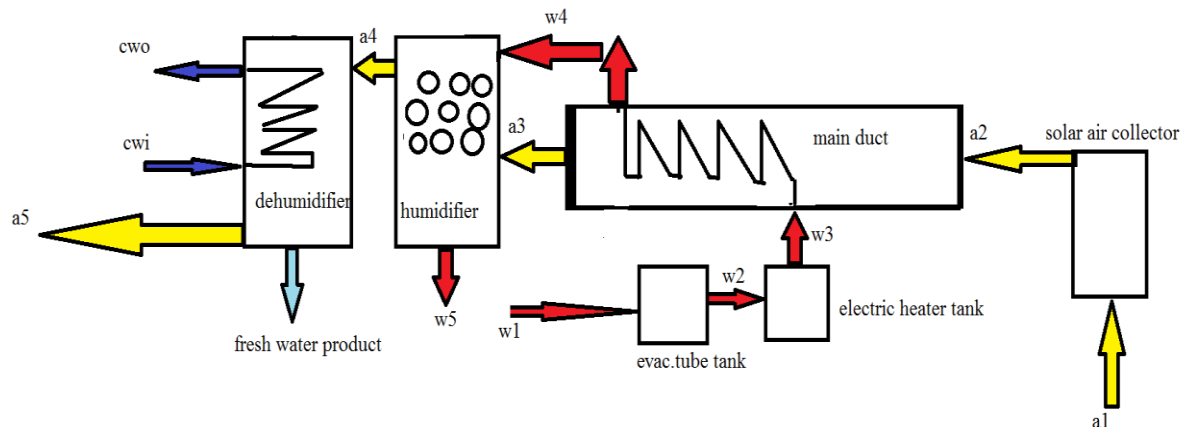
Fig. 4: HDH desalination system layout.
