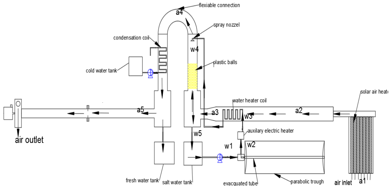
Fig. 1: A diagram of the setup.
