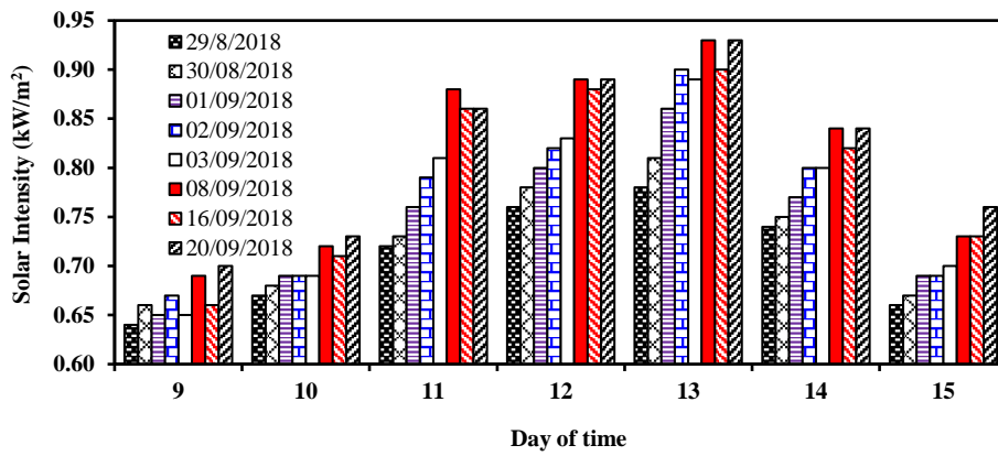
Fig. 5: Solar radiation intensity from 9 A.M. to 3 P.M.
