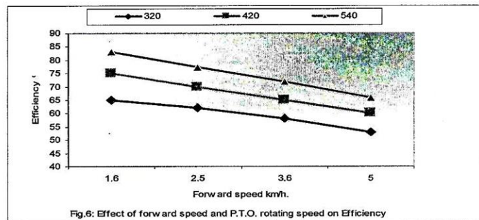
Fig.6: Effect of forw ard speed and P.T.O. rotating speed on Efficiency
