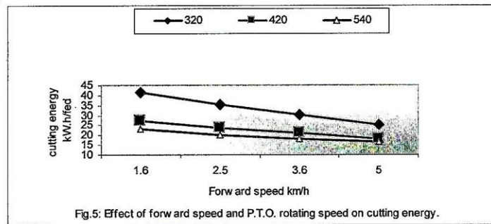
Fig.5: Effect of forw ard speed and P.T.O. rotating speed on cutting energy.
