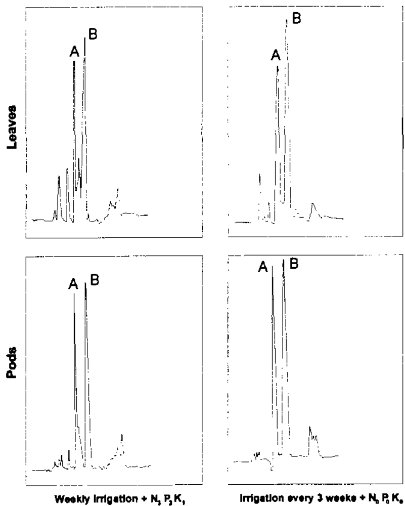
Fig. (1): HPLC analysis of glycosides extracted from leaves and pods of senna ( Cassia acutifolia , Delile) plants irrigated weekly and fertilized with N 2 P 2 K 1 , or irrigated every 3 weeks and receiving no fertilization (N 0 P 0 K 0 ).
